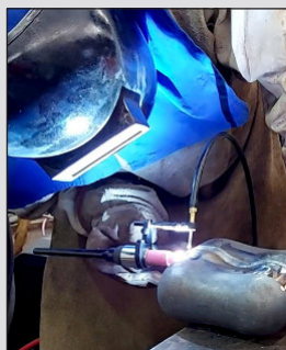
TOCHA TIG MANUAL
